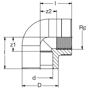
621.10.02 PVC-U Ü-Winkel 90° IG-zyl grau PVC-U Transition-Elbow 90° female-thread-cyl grey
