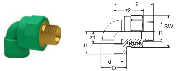
G 8092gB PP-RCT-RG Ü-Winkel 90° AG-keg grün PP-RCT-Bronze Transition-Elbow 90° male-thread-con green
