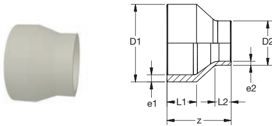
BG 89101 PP-INDUSTRIAL Reduktion kurz st SDR11 grau PP-INDUSTRIAL Reducer short butt SDR11 grey
