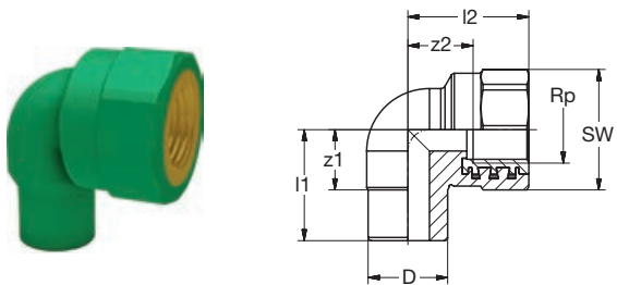
G 8091gB PP-RCT-RG Ü-Winkel 90° i IG-zyl grün PP-RCT-Bronze Transition-Elbow 90° fem female-thread-cyl green
