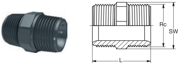
621.91.19 PVC-U Doppelnippel AG-keg grau PVC-U Hexagon nipple male-thread-con grey
