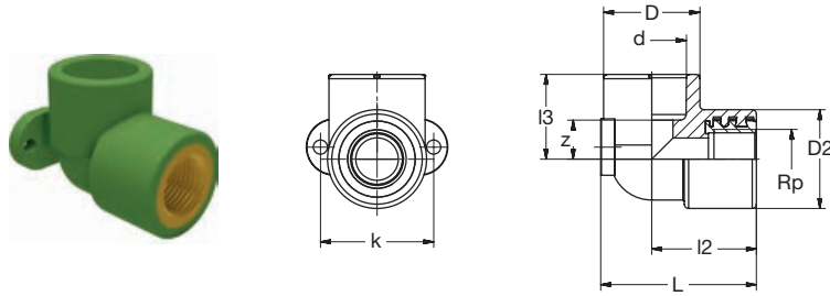
G 8472g PP-R-RG Ü-Winkel 90° Wandbefestigung IG-zyl grün PP-R-Bronze Transition-Elbow 90° wall mount female-thread-cyl green
