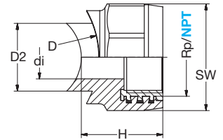
G 8270s PP-RCT-RG Einschweißsattel IG-zyl grün PP-RCT-Bronze Weld-in-saddle female-thread-cyl green
