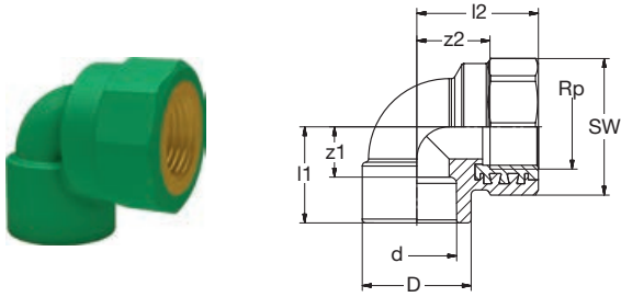
G 8090gB PP-RCT-RG Ü-Winkel 90° IG-zyl grün PP-RCT-Bronze Transition-Elbow 90° female-thread-cyl green
