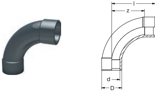
621.00.01 PVC-U Bogen 90° grau PVC-U Bend 90° grey
