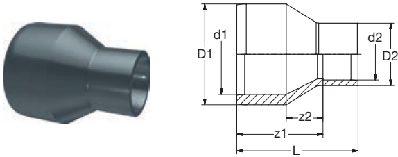
621.91.03 PVC-U Reduktion lang grau PVC-U Reducer long grey
