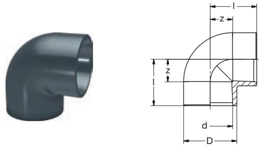
621.10.01 PVC-U Winkel 90° grau PVC-U Elbow 90° grey
