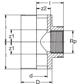
621.20.02 PVC-U Ü-T-Stück 90° IG-zyl grau PVC-U Transition-Tee 90° female-thread-cyl grey
