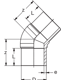
G 8041B PP-RCT Winkel 45° lang st SDR11 grün PP-RCT Elbow 45° long butt SDR11 green
