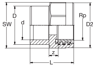
620.91.02 PVC-U-RG Übergang IG-zyl grau PVC-U-Bronze Transition female-thread-cyl grey
