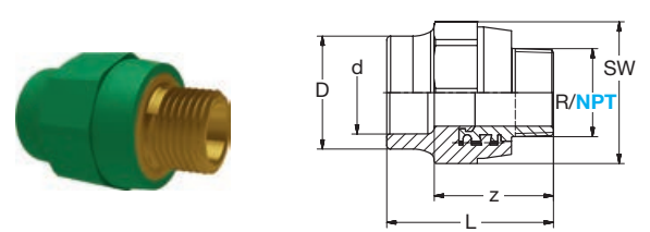
G 8243gB PP-RCT- RG Übergang AG-keg grün PP-RCT- Bronze Transition male-thread-con green
