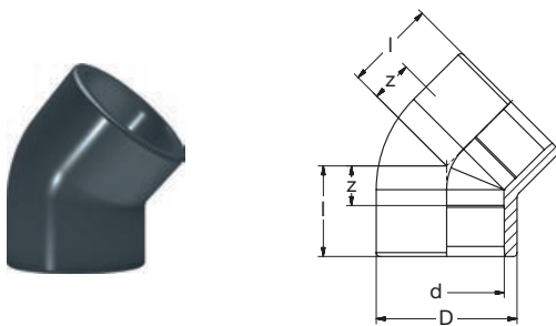
621.15.01 PVC-U Winkel 45° grau PVC-U Elbow 45° grey
