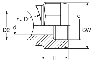
G 8130s PP-RCT Einschweißsattel Muffe grün PP-RCT Weld-in-saddle socket green
