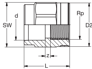
621.91.02 PVC-U Übergang IG-zyl grau PVC-U Transition female-thread-cyl grey
