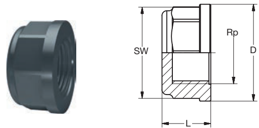
621.96.06 PVC-U Kappe IG-zyl grau PVC-U Cap female-thread-cyl grey
