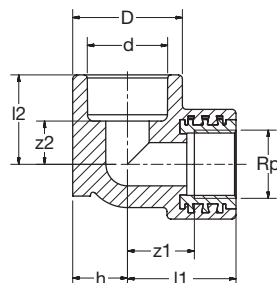
620.100 PVC-U-RG Ü-Winkel 90° IG-zyl Wandbefestigung grau PVC-U-Bronze Transition-Elbow 90° female-thread-cyl wall-mount grey
