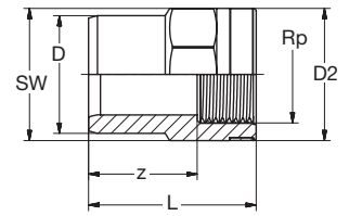
621.91.04 PVC-U Ü-Reduktion IG-zyl grau PVC-U Transition-Reducer female-thread-cyl grey
