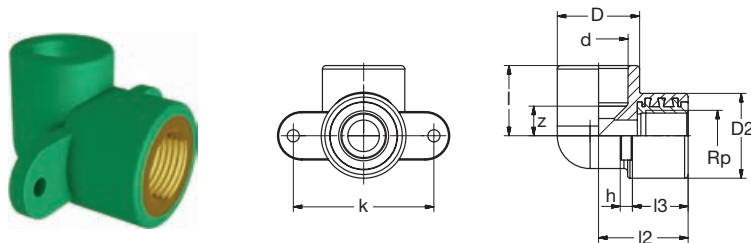
G 8473gB PP-RCT-RG Ü-Winkel 90° Hohlwandbefestigung IG-zyl grün PP-RCT-Bronze Transition-Elbow 90° hollow wall mount female-thread-cyl green
