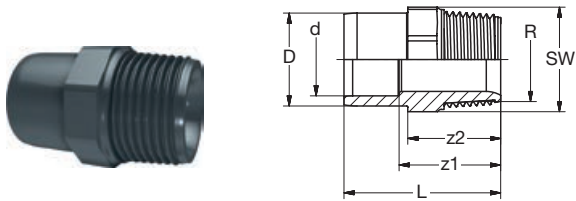
621.91.17 PVC-U Ü-Reduktion/Muffe AG-keg grau PVC-U Transition-Reducer/Socket male-thread-con grey
