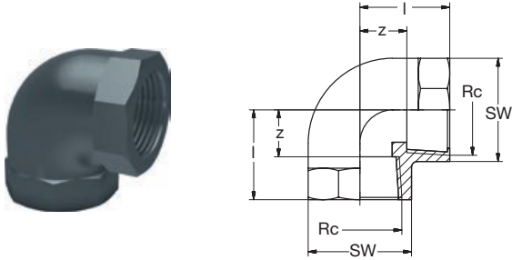
621.10.16 PVC-U Winkel 90° IG-keg grau PVC-U Elbow 90° female-thread-con grey
