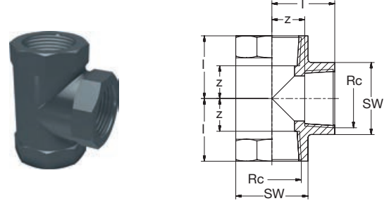
621.20.16 PVC-U T-Stück 90° IG-keg grau PVC-U Tee 90° female-thread-con grey
