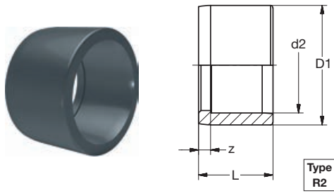
621.90.03 PVC-U Reduktion kurz grau PVC-U Reducer short grey
