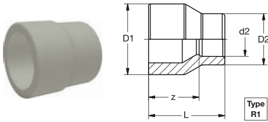
BG 8243 PP-INDUSTRIAL Reduktion grau PP-INDUSTRIAL Reducer grey
